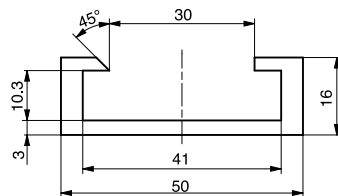
Plastic C profile for flat steel, 50 × 6 extruded
